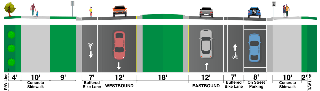
Typical Section between Douglas Ave and Highland Ave
